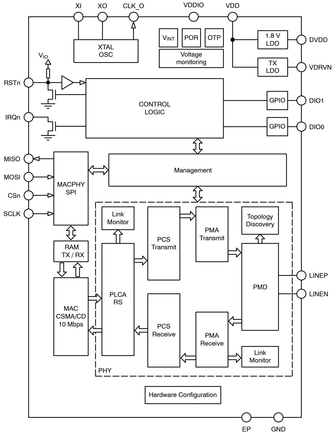
Figure 2. Block Diagram
